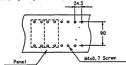
Fig.8 Panel (Wall) Mounting Dimension
