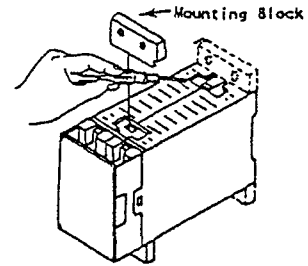
Fig.6 Mounting Block installation and removal
