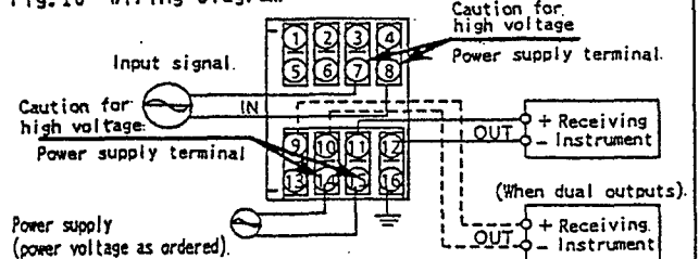
Fig.10 Wiring Diagram
